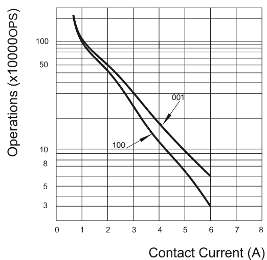
ENDURANCE CURVE
